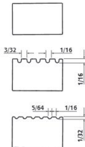
17610 U Notch Economy : 3/32" x 1/16" x 1/16" For use on sheet vinyl with porous subfloors(wood and concrete).
